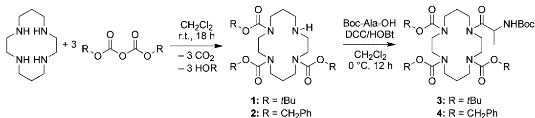
Scheme 2. Synthesis of the Boc- and Cbz-protected Boc-( S )-alanyl cyclam derivatives Boc-( S )-Ala-cyclam-Boc 3 ( 3 ) and Boc-( S )-Ala-cyclam-Cbz 3 ( 4 ).
