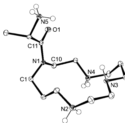
Figure 1. ORTEP plot at 50% probability of the cation Alanyl-cyclam· 3\text{H}^+ ( 5 ) (hydrogen atoms except for NH are omitted for clarity); selected bond lengths [pm], angles [ ^\circ ], \tau [ ^\circ ], and \chi_N [ ^\circ ]: C11–N1 135.7(2), C11–O1 123.3(2); C1–N1–C10 118.1(2), C1–N1–C11 124.3(2), C10–N1–C11 115.3(2); \tau = 9.3 ; \chi_N = 17.7 .
