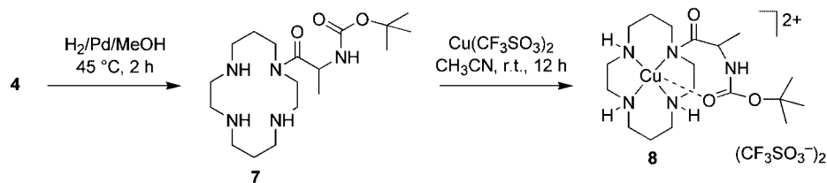
Scheme 4. Hydrogenation of the Cbz-protected compound 4 to the free ligand 7 and synthesis of the copper complex [\{\text{Boc-(S)-Ala-cyclam}\}\text{Cu}](\text{CF}_3\text{SO}_3)_2 ( 8 ).
