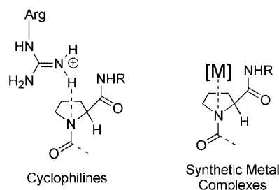
Scheme 1. Electrophilic activation of a tertiary amide group; hydrogen bonding in peptides and proteins (left), or metal coordination (right).
