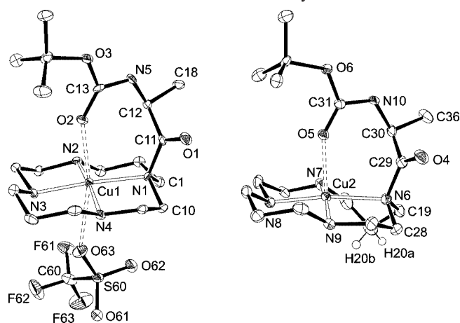
Figure 2. ORTEP plots at 50% probability of the two complexes A and B observed in the structure of [\{\text{Boc-(S)-Ala-cyclam}\}\text{Cu}](\text{CF}_3\text{SO}_3)_2 ( 8 ) (hydrogen atoms except for those located at C20 in complex B , and the three non-coordinating triflate ions are omitted for clarity); selected distances [pm], angles [°], \tau [°], and \chi_N [°] of A : Cu1–N1 212.7(3), Cu1–N2 201.2(3), Cu1–N3 202.1(3), Cu1–N4 200.5(3), Cu1–O2 248.8(2), Cu1–O63 278.9, C11–N1 146.9(4), C11–O1 120.2(4); N1–Cu1–N2 95.3(2), N1–Cu1–N3 175.7(2), N1–Cu1–N4 86.7(2), N1–Cu1–O2 92.4(2), N2–Cu1–N3 86.7(2), N2–Cu1–N4 170.3(2), N2–Cu1–O2 92.7(2), N3–Cu1–N4 90.7(2), N3–Cu1–O2 91.4(2), N4–Cu1–O2 96.7(2), Cu1–N1–C1 112.4(2), Cu1–N1–C10 100.6(2), Cu1–N1–C11 112.8(2), C1–N1–C10 109.8(3), C1–N1–C11 112.8(2), C10–N1–C11 109.3(2); \tau = 35.8; \chi_N = 58.5; selected distances [pm], angles [°], \tau [°], and \chi_N [°] of B : Cu2–N6 214.7(3), Cu2–N7 203.1(3), Cu2–N8 200.9(3), Cu2–N9 202.1(3), Cu2–O5 230.5(2), Cu2–H20b 270.5, C29–N6 146.2(5), C29–O4 119.9(5); N6–Cu2–N7 96.3(2), N6–Cu2–N8 172.02(2), N6–Cu2–N9 85.3(2), N6–Cu2–O5 92.2(2), N7–Cu2–N8 85.5(2), N7–Cu2–N9 165.7(2), N7–Cu2–O5 97.3(2), N8–Cu2–N9 91.1(2), N8–Cu2–O5 93.3(4(2), N9–Cu2–O5 96.8(2), Cu2–N6–C19 112.5(2), Cu2–N6–C28 102.6(2), Cu2–N6–C29 109.2(2), C19–N6–C28 110.4(3), C19–N6–C29 110.9(3), C28–N6–C29 111.1(2); \tau = 30.6; \chi_N = 56.9.
