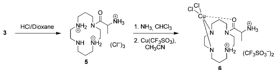
Scheme 3. Acid deprotection of Boc-( S )-Ala-cyclam-Boc 3 ( 3 ) and the reaction of Ala-cyclam·3HCl ( 5 ) with copper(II) triflate.
